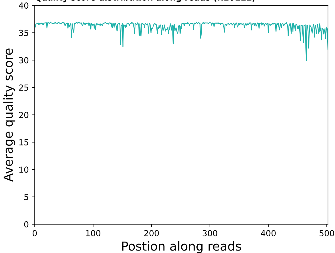
Quality score distribution along reads (R10111)
